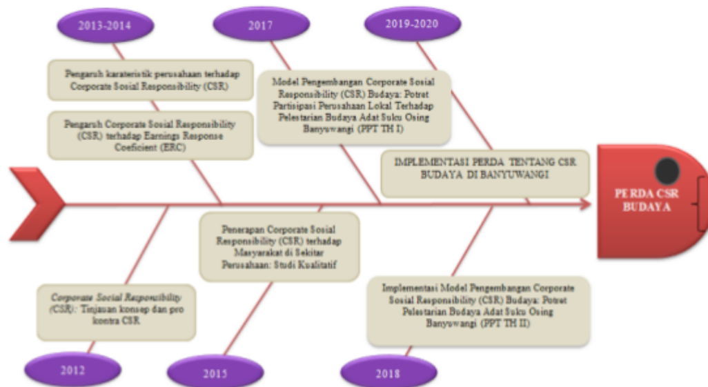
Gambar 1. Fishbone Diagram
