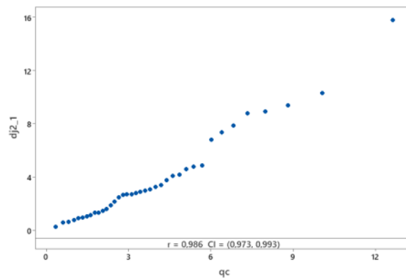
Figure 1. Multivariate Normal Probability Plot
