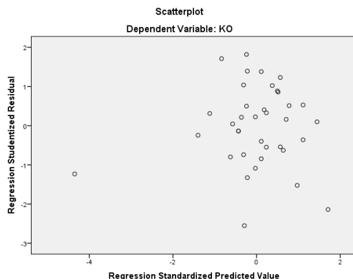
Figure 2. Scatterplot Heteroskedastissity Test
