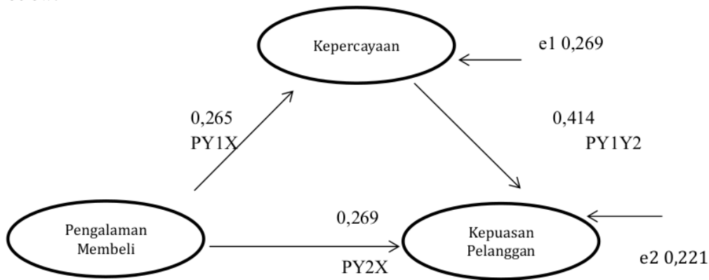
Figure 2. The Path Equation Model
